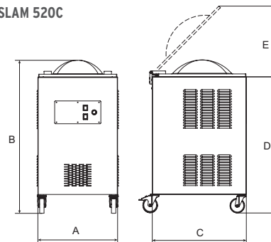
SLAM 520C
